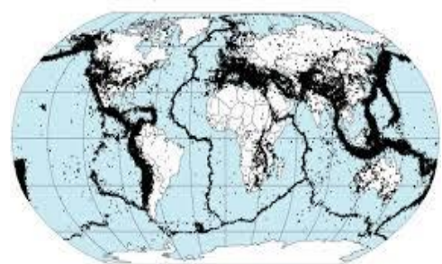
Preliminary Determination of Epicenters 358,214 Events, 1963 - 1998
