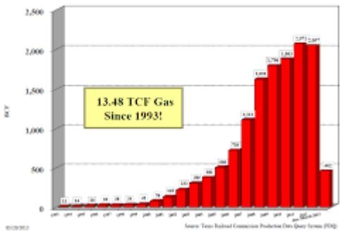
Newark, East (Barnett Shale) Total Natural Gas Production 1993 through March 2013
