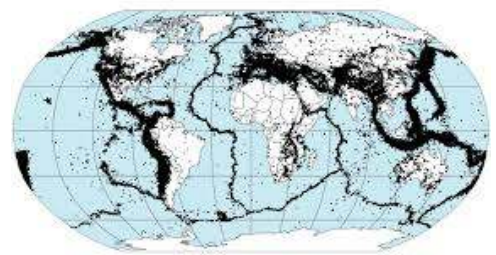
Preliminary Determination of Epicenters 358,214 Events, 1963 - 1998
